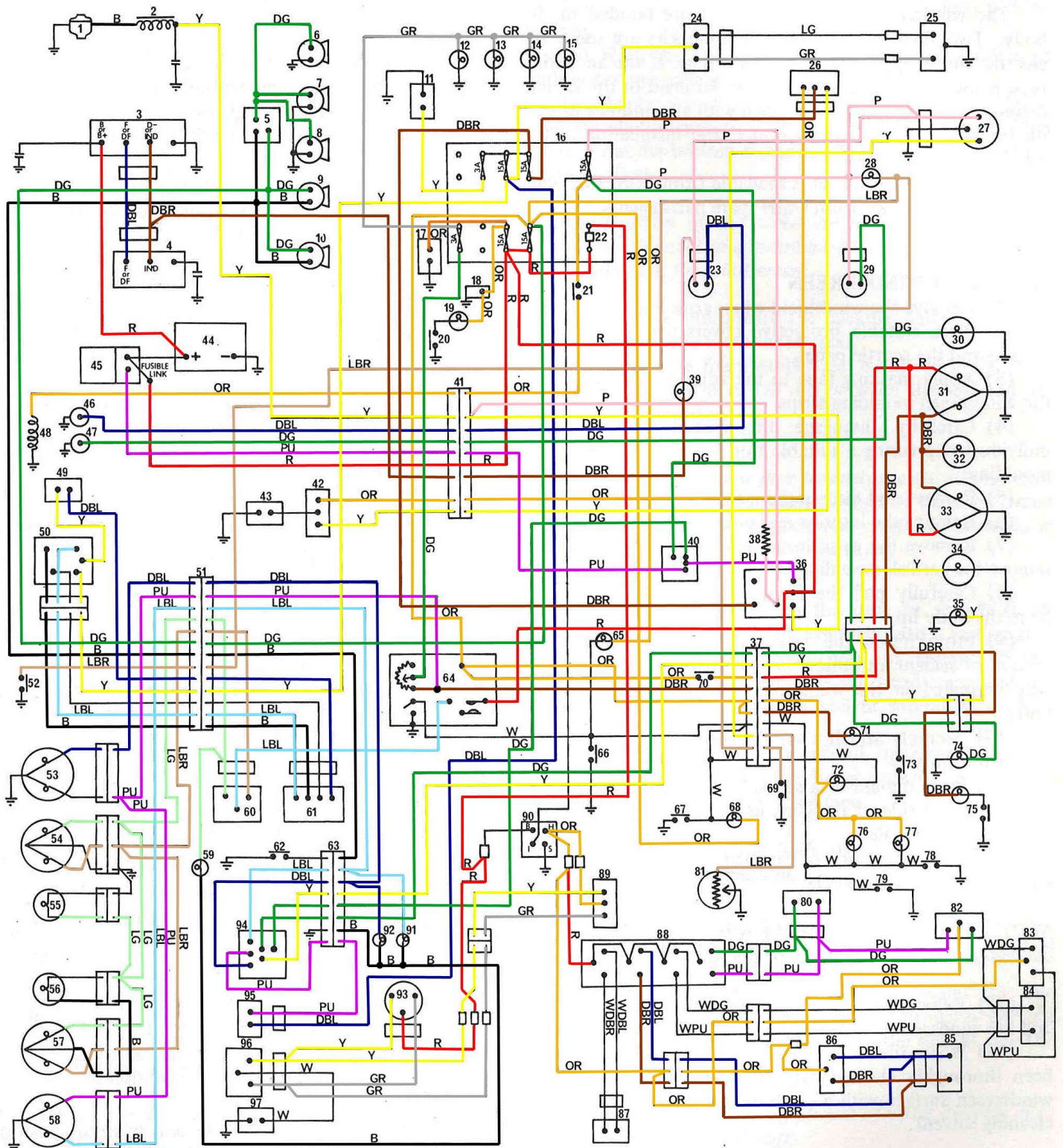
Wiring Diagram for Statesman de Ville.
